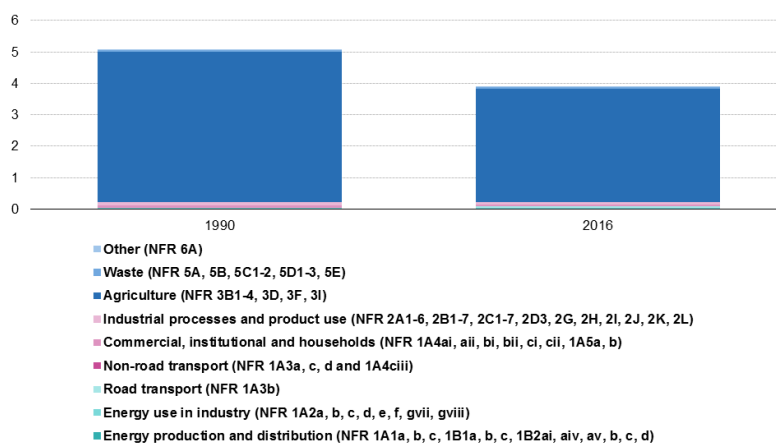
Emissions of ammonia by source sector, EU-28, 1990 and 2016 (Million tonnes)
