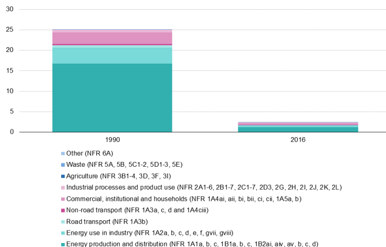
Emissions of sulphur oxides by source sector, EU-28, 1990 and 2016 (Million tonnes)
