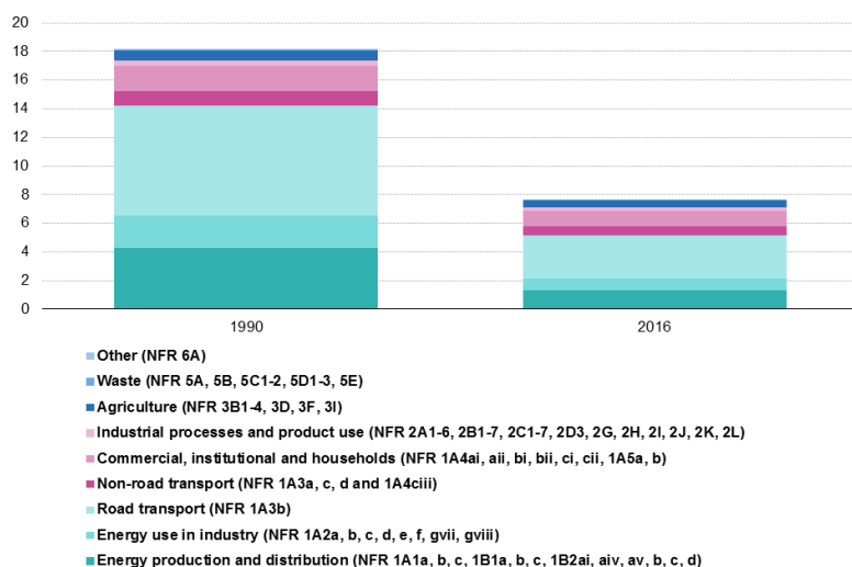
Emissions of nitrogen oxides by source sector, EU-28, 1990 and 2016 (Million tonnes)
